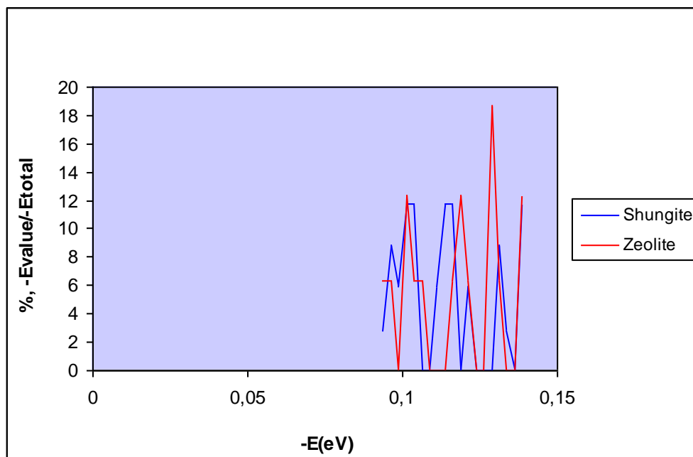
Figure 3. The distribution [%, (-E_{\text{value}})/(-E_{\text{total value}}) ] of water molecules in water solution of shungite/zeolite according to energies of hydrogen bonds ( -E_{\text{value}} ) to total result of hydrogen bonds energy
